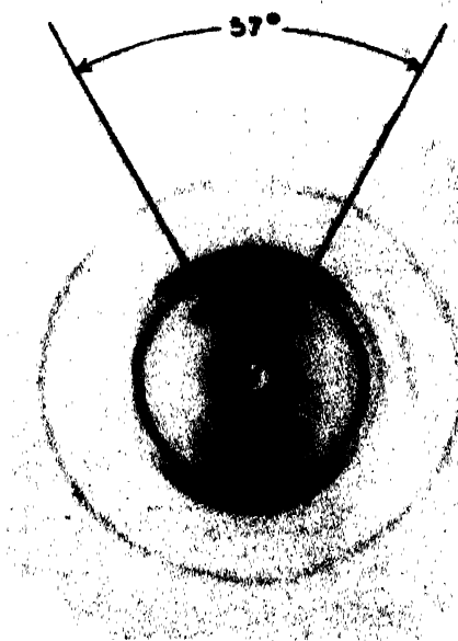
FIG. 8. X-RAY FIBER DIAGRAM OF UNSTRETCHED MATURE COTTON. (COURTESY OF W. A. SISSON.)
